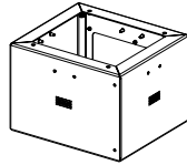
288 PON 12" Riser
